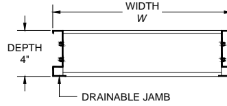
MODEL: 2450 FRAME: CHANNEL FRAME DUCT-MOUNT (DM)
